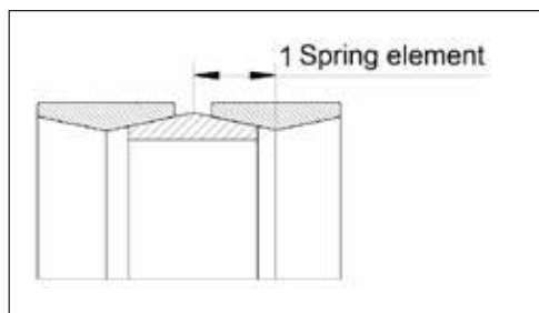
Fig. 3: Drawing 2 outer rings and 1 inner ring
