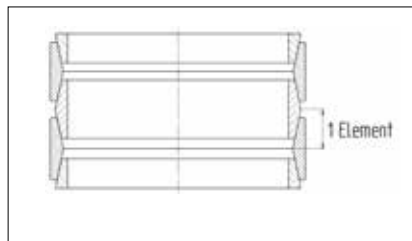
Fig. 1: Friction spring with 4 elements
