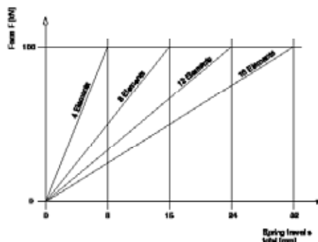
Fig. 4: Characteristic curve changeable by selection of ring number
