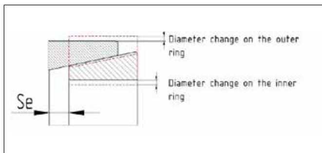
Fig. 2: Friction spring with diameter deviation
