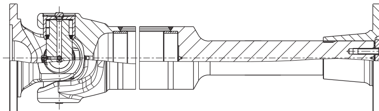
Pumpenwelle / Pump shaft
